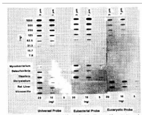
FIG. 3. Small-subunit rRNA-based hybridization of nucleic acids extracted from sediment samples.
