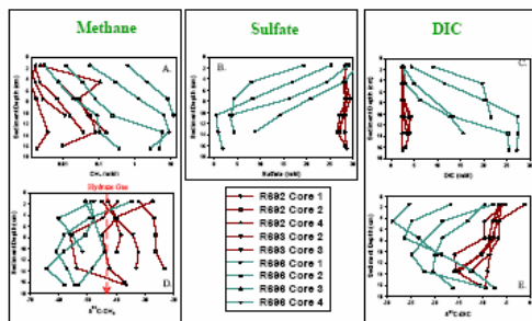
Figure 4. Concentration and stable isotope profiles from push cores collected in Barkley Canyon during June 2003. The open lines represent push cores with evidence for anaerobic oxidation of methane (AOM). Red lines represent cores with low methane concentrations and no indication of AOM. The vertical line in Fig. 4D represents the \delta^{13}\text{C} of methane from Barkley Canyon hydrate gas.
