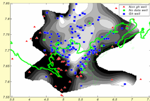
Figure 1: Location of wells with and without inferred gas hydrates as well as the inferred GH thickness map (metres) of the BMB, with the coast of the Beaufort Sea for geographical reference.
