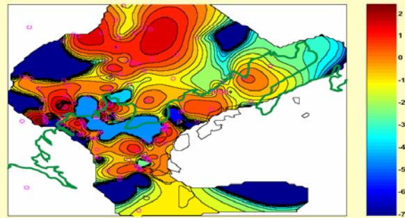
Figure 4: GH resource potential map resulting from the deterministic resource assessment (logarithmic value GH yield map, i.e. scaled to show low GH yields), with the coastline of the Beaufort Sea shown for geographical reference.
