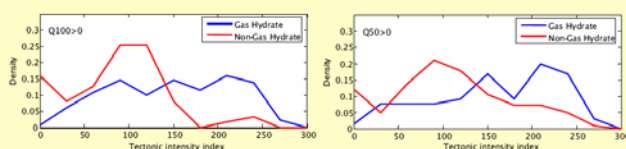
Figure 3a and 3b: Probability densities of Tectonic intensity index for GH and non-GH wells for all (left) and right (Sgh>50%, right) GH occurrences.
