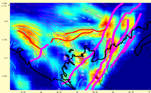
Figure 2: Tectonic intensity index (i.e., fault and fold density) map for the BMB, a geological proxy indicator for gas migration into the GHSL, with the coast of the Beaufort Sea for geographical reference.
