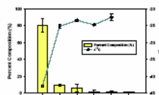
Figure 3. Hydrocarbon and stable isotope composition of Barkley Canyon hydrate gas. High concentrations of \text{C}_2 - \text{C}_{10} hydrocarbons and ^{13}\text{C} -depleted methane ( \text{C}_2 - \text{C}_{10} ) are clear indicators for a thermogenic gas source.
