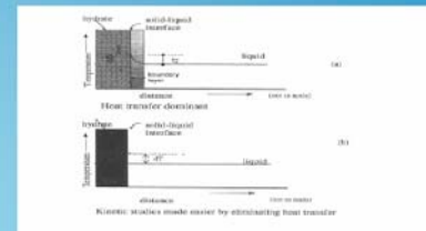
Figure 3.2: Schematic for Heat Transfer Effects
