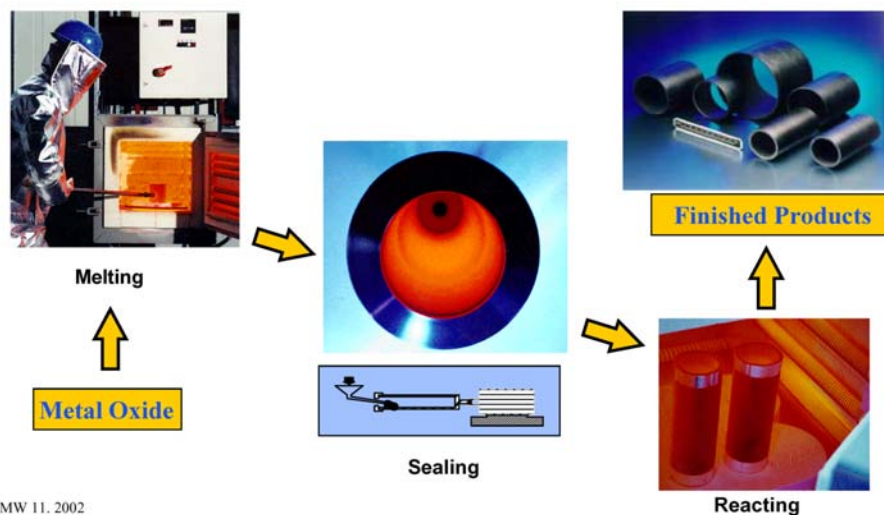
Figure 2.2-6 Production Process of BSCCO Melt Textured Material
