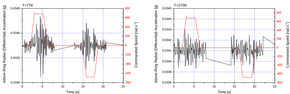
Figure 3.3-4 Niobium Above-Ring Radial Differential Sensor Comparison at 77K and 270K
