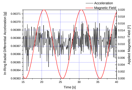
Figure 3.2-4 Influence of Magnetic Field on In-Ring Radial Sensor with BSCCO at 77K and 270K
