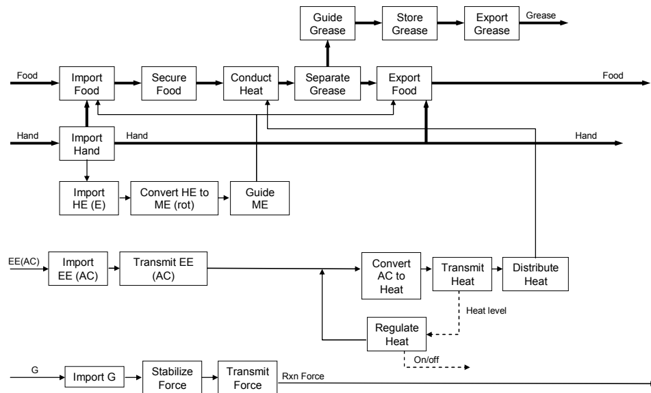
Grill Initial Functional Model
