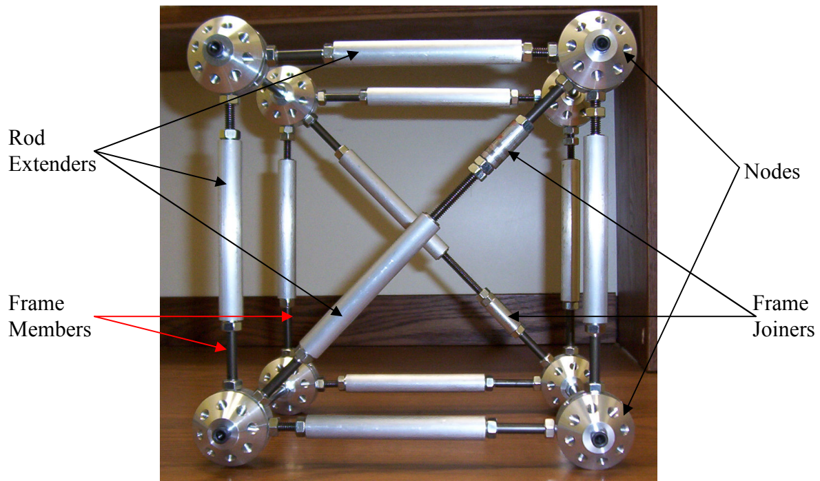
Figure 51: Structural Box
