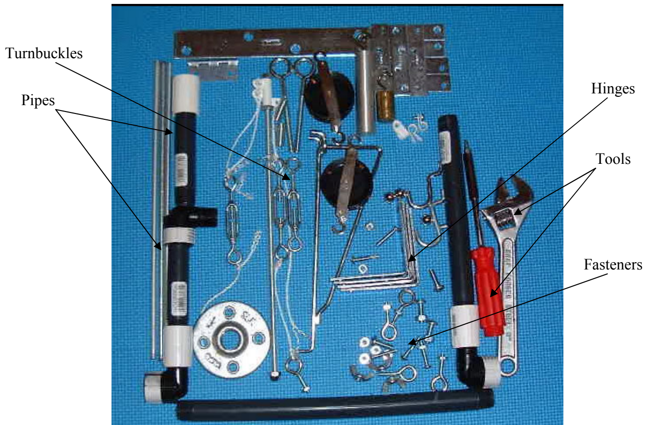
Figure 16: Parts included with Pegboard Mechanical Breadboard (Van, 2004)
