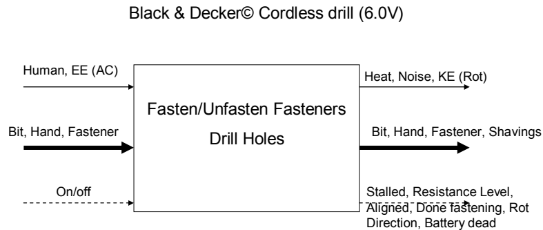
Figure 19: Black Box Cordless Screwdriver Model
