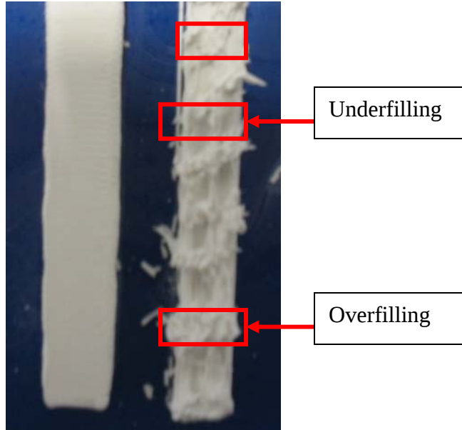
Figure 7: Top view of bars fabricated using extrusion force controller (left) and constant ram velocity (right, v = 2 \mu\text{m/sec} ).
