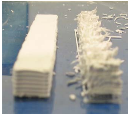
Figure 8: Side view of bars fabricated using extrusion force controller (left) and constant ram velocity (right, v = 2 \mu\text{m/sec} ).
