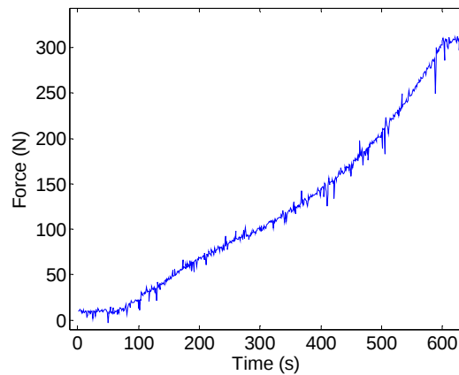
Figure 9: Extrusion force time history for test bar made with constant ram velocity ( 2 \mu\text{m/sec} ).
