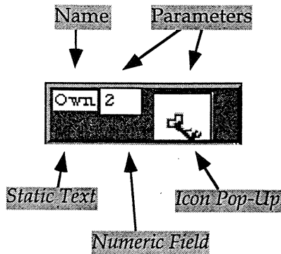
Figure 5: A Visual AgenTalk Command
