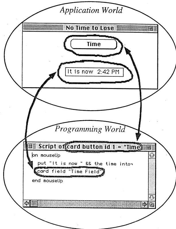
Figure 1: A HyperCard Example
