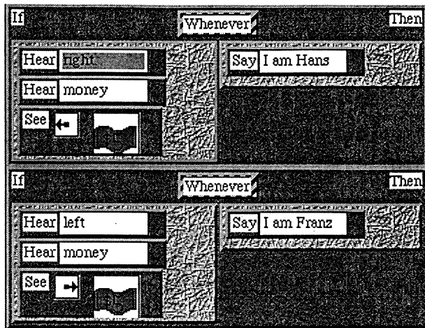
Figure 23: Rules for Listeners
