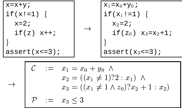
Figure 6: Example: Renaming and transformation. The first box on the left contains the unwound program with assertions. Each variable is a bit vector. The first step is to rename the variables. Then the program is transformed into a bit vector equation as described in section 3.6.
