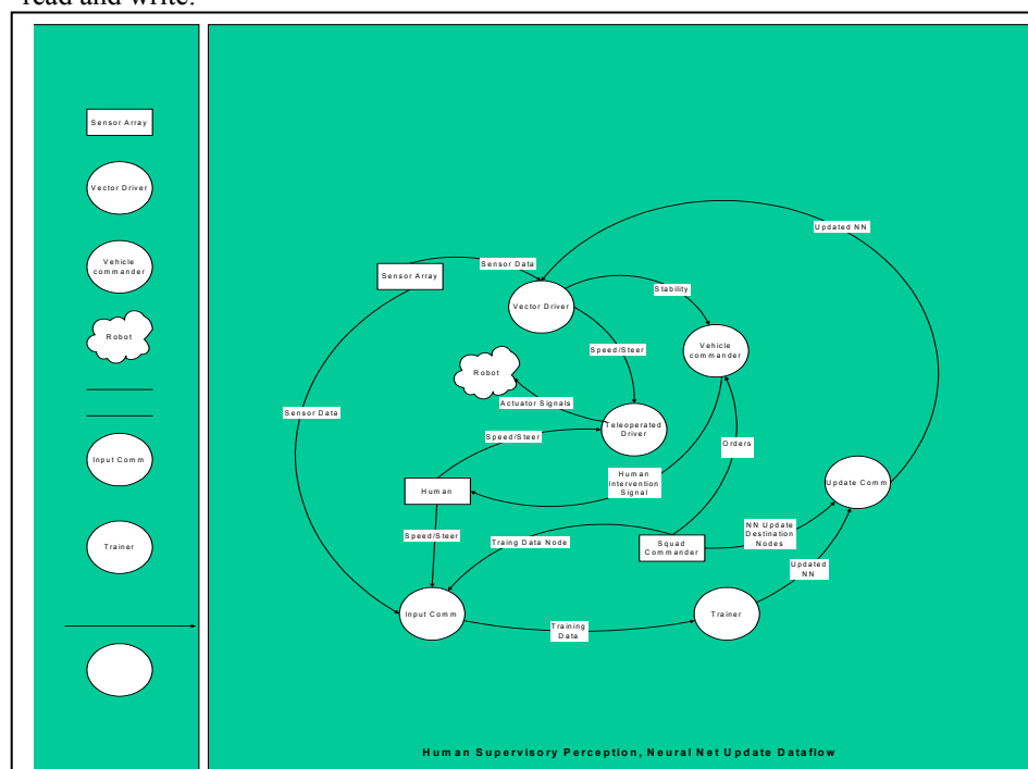
Figure 10 Model for Prototype GUI
