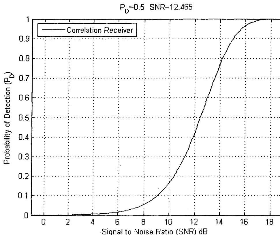
Figure 3. Predicted performance of a correlation receiver calculated using a transmission loss pdf like that shown in Figure 2. The P_{FA} is 10^{-4} .
