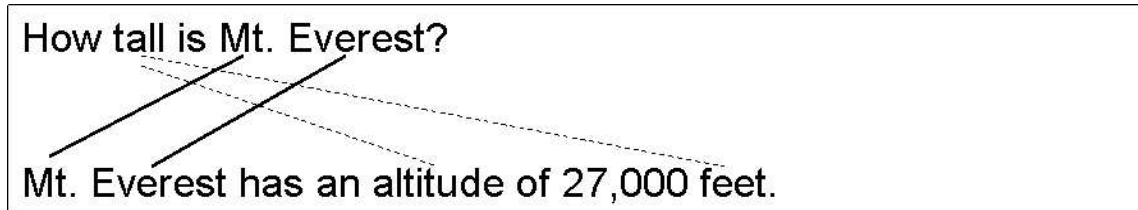
Figure 4.2. A question and answer pair, with dotted lines representing possible word pairs in a translation table. Solid lines represent matching words which have been given a probability 1.0.
