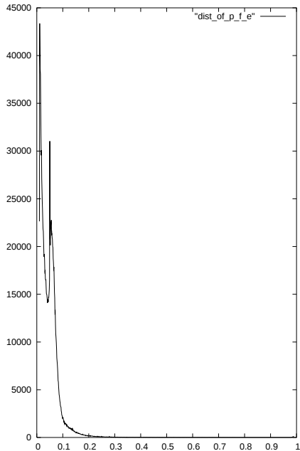
Figure 4.3. The distribution of probabilities in the translation table for IBM model 3 learned from a corpus of query-sentence pairs artificially constructed from newswire text, as described in [95]. The x-axis is the value of the probability. The y-axis is the number of times that probability occurred in the translation table.
