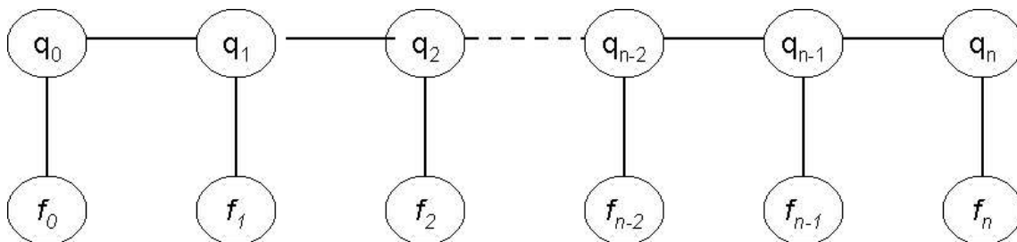
Figure 5.3. The graphical model for question-answering conditional models. The label sequence is the sequence of question words. Each question token has a feature vector associated with it that are computed over the entire answer sentence.
