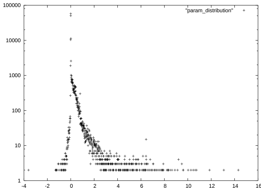
Figure 5.5. The distribution of parameters in the models trained on “What” and “How” questions. Parameter values that only occur once have been omitted.
