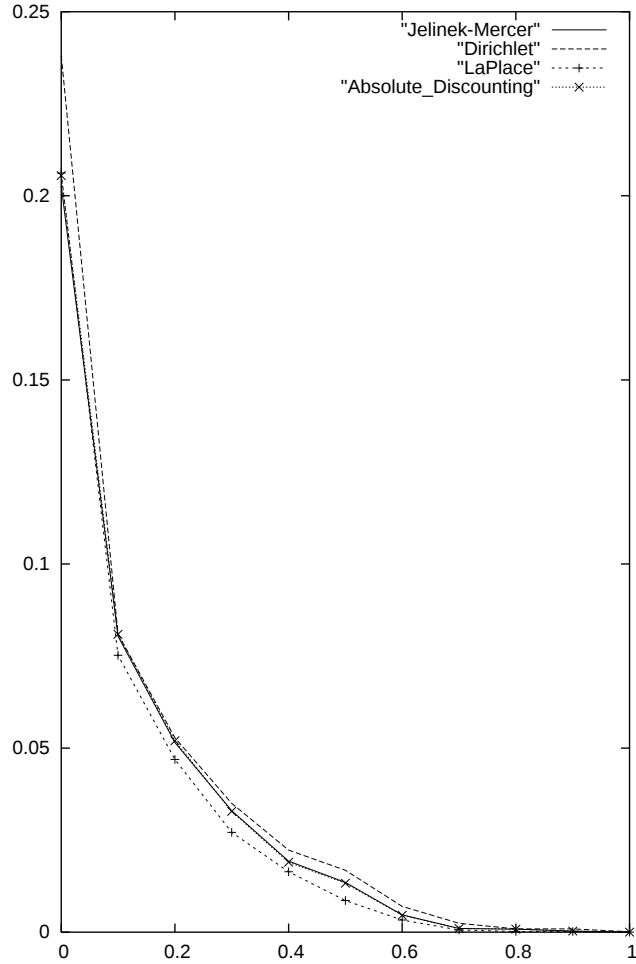
Figure 2.2. Comparing smoothing strategies for sentence retrieval on TREC-style topic titles. There was no significant difference between smoothing strategies, except that the result for LaPlace smoothing for topic descriptions was significantly worse using a Wilcoxon sign test at the p < .05 level.
