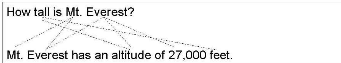
Figure 4.1. A question and answer pair, with dotted lines representing possible word pairs in a translation table under the assumptions of Model 1.
