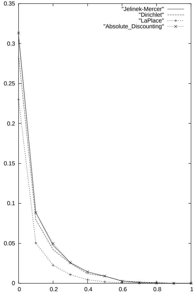
Figure 2.1. Comparing smoothing strategies for sentence retrieval on TREC-style topic descriptions. There was no significant difference between smoothing strategies, except that the result for LaPlace smoothing for topic descriptions was significantly worse using a Wilcoxon sign test at the p < .05 level.
