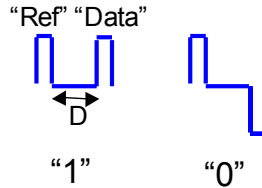
Figure 6. TR modulation technique
