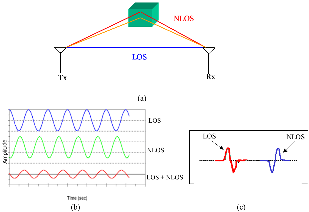
Figure 5. (a) Multipath phenomenon in wireless channels (b) Multipath effect on narrowband signals (c) multipath effect on ultra-wideband pulses
