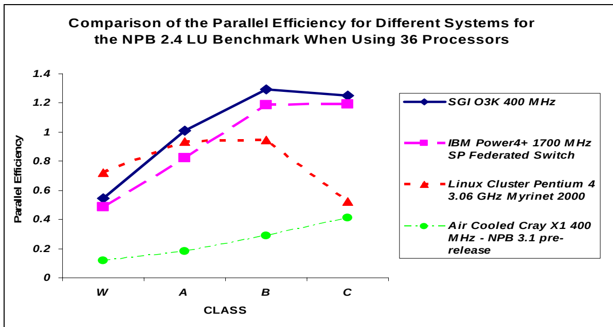
Figure 12. Comparison of the parallel efficiency for different systems for the NPB 2.4 LU benchmark when using 32 processors.
