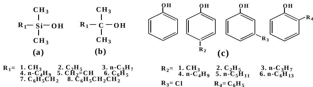
Fig. 1. Chemical structures (a) Alkyl dimethylsilanols (b) Alkyl dimethylcarbinols, (c) Substituted phenols
