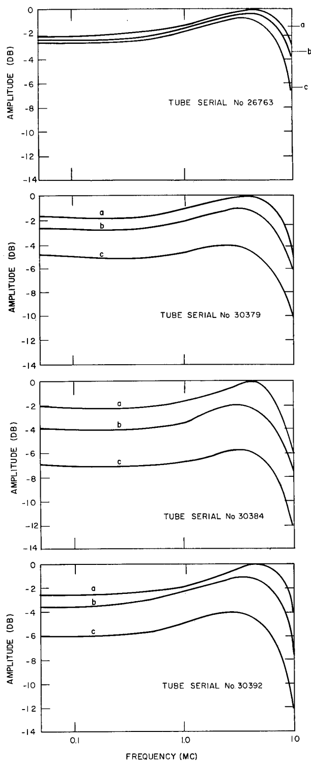
Fig. 2 - Noise spectra of sample 6700 type counter tubes. Target currents were (a) 7 milliamps, (b) 5 milliamps, and (c) 3 milliamps
