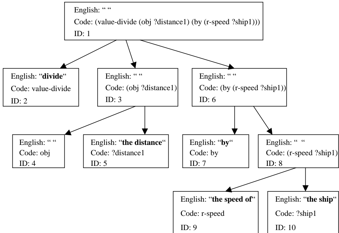
Figure 4: Tree structure for an EXPECT method body fragment.
