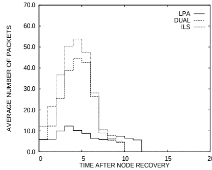
Fig. 9. Average number of packets for Node Recovery
