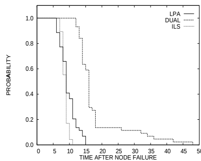
Fig. 6. Probability of packets in transit for Node Failure
