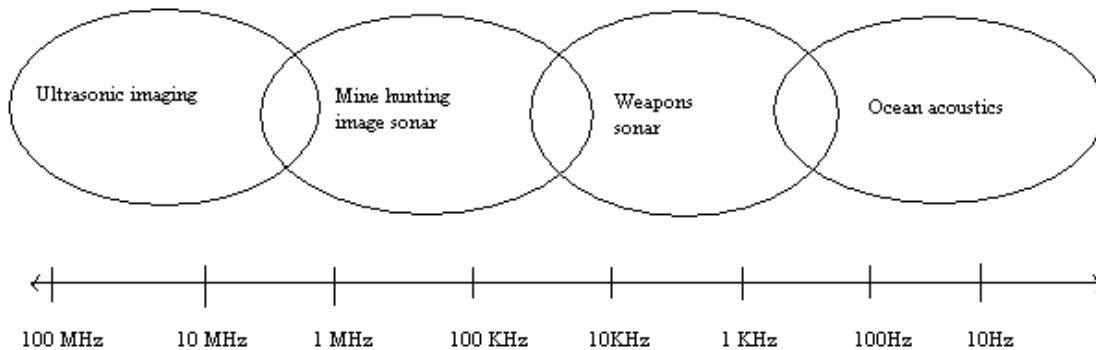
Figure 2.1 Transducers for different acoustic frequency range.
