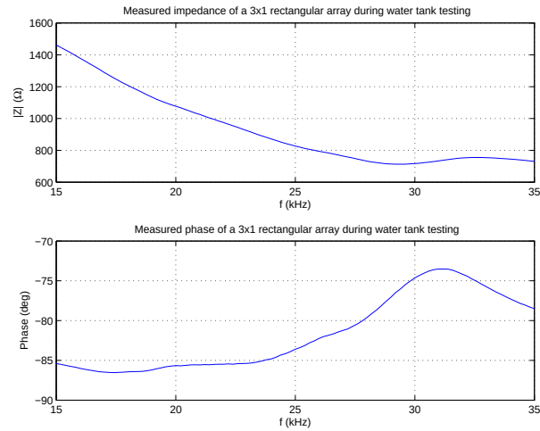
Figure C.8: Measured impedance magnitude and phase of a 3x1 rectangular array
