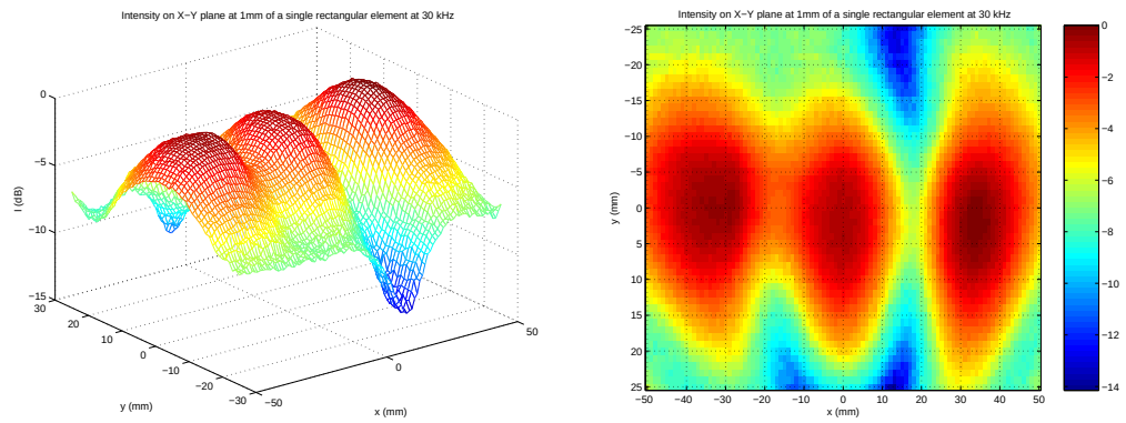
Figure C.12: Exposimetry of a single element rectangular cymbal transducer array 1 mm from the transducer face at 30 kHz
