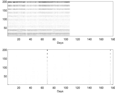
Figure 5: Abnormal Dynamics Discovered by Clustering
