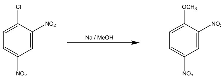
Scheme 1. Synthesis of DNAN from 1-chloro-2,4-dinitro benzene (DNCB).
