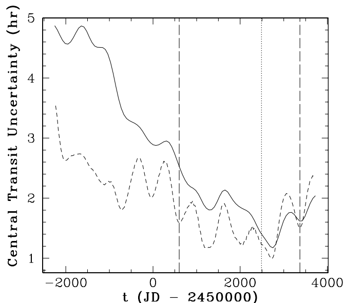
FIG. 1.— Uncertainty in the central transit time for planets Gl 876b (solid line) and Gl 876c (dashed line). The vertical dashed lines delineate the time span of the Keck RV observations used to generate the coplanar fits that form the basis of our model photometric and RV curves. The vertical dotted line indicates the epoch for the fits (JD 2,452,490.0).
