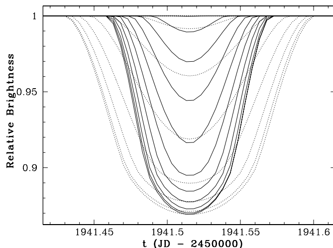
FIG. 3.— Model transit light curves for planet Gl 876c, when it is near periastron (solid curves), and near apastron (dotted curves). Inclinations, i = 90^\circ through i = 89^\circ 0' are shown in decrements of 0.1^\circ . Planet Gl 876c's eccentricity e \sim 0.22 leads to a greater difference in transit depth and duration between periastron and apastron.
