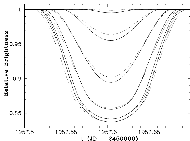
FIG. 2.— Model limb-darkened light curves during a predicted transit by planet Gl 876b when it is near periastron (solid curves) and near apastron (dotted curves). The curves correspond to different assumed inclinations ( i = 90^\circ, 89^\circ 9', 89^\circ 8', \dots, 89^\circ 5' ). The shallowest occur for i = 89^\circ 5' .
