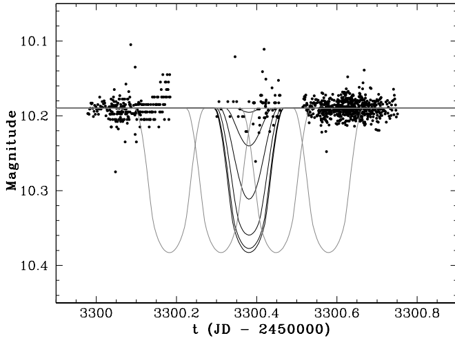
FIG. 10.—Dynamical model light curves for Gl 876 due to planet b for i = 90^\circ 0 through 89^\circ 5 in 0^\circ 1 decrements, near a predicted transit centered at JD 2,453,300.3806. As with the previous figure, the data were baselined and shifted to employ a mean magnitude of V = 10.19 , based on relative photometry obtained by AAVSO and Transitsearch (filled circles). The light lines correspond to i = 90^\circ model light curves arising from bootstrap fits in which the transit is 3\sigma early, 1\sigma early, and 1\sigma late and 3\sigma late.
