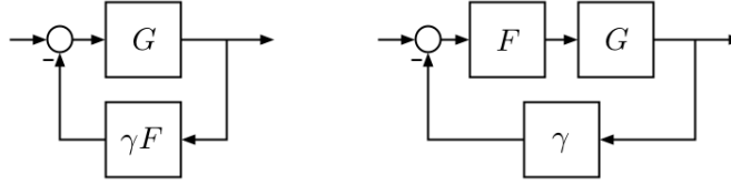
Fig. 1. Left: The spatially periodic closed-loop system as the feedback interconnection of a spatially invariant system G and a spatially periodic multiplication operator F . Right: The closed-loop system \mathbf{S}^{\text{cl}} in the standard form for Nyquist stability analysis.
