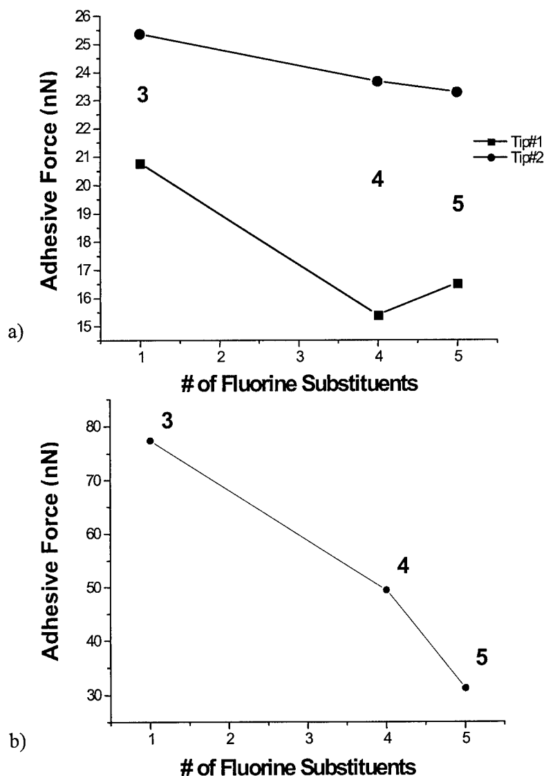
Figure 7. Interfacial adhesion measured between (a) aromatic thiol-SAMs and \text{Si}_3\text{N}_4 tip, and (b) between aromatic thiol-SAMs and Au-coated Si tip measured under static conditions.
