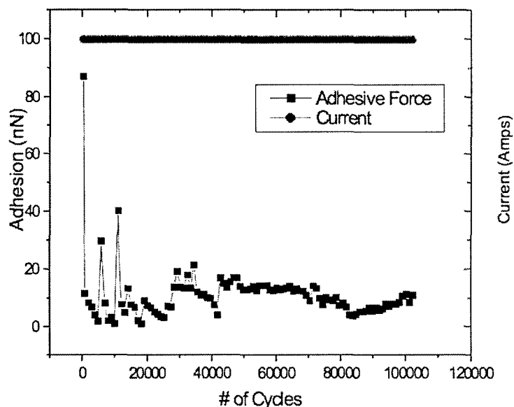
Figure 6. Simultaneous adhesion and current measurements performed with AFM under continuous flow of fluorinated thiol.
