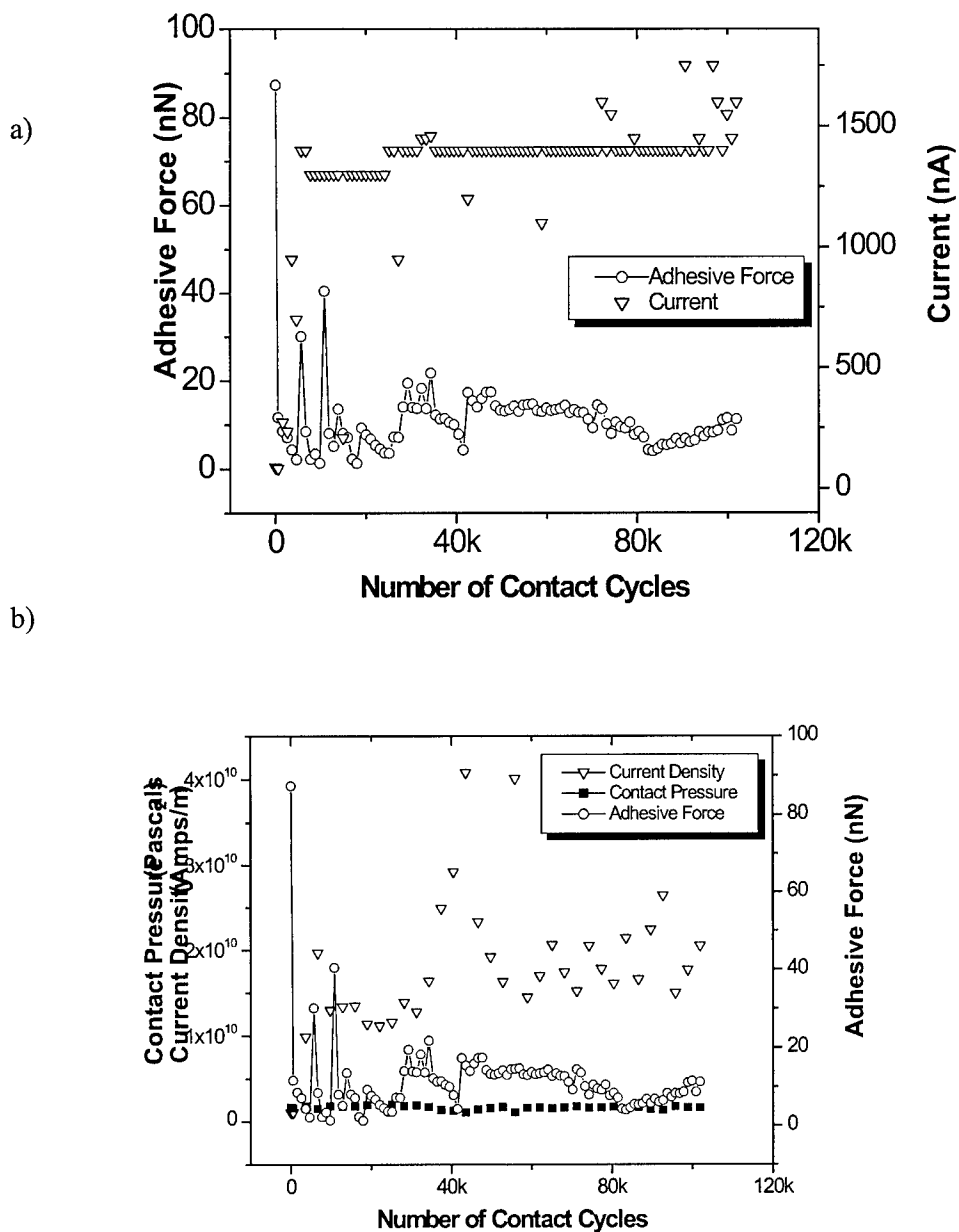
Figure 8. Current flow and adhesion measured with a 0.30 V bias between a gold-coated AFM tip and a gold substrate as a function of the duration of flow of vapors of C_7H_7FS . The graph shows a significant decrease in adhesion was achieved while current was sustained between the two metal electrodes for over 100,000 switching cycles.
