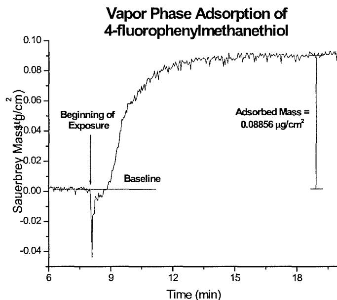
Figure 2. QCM measurement of vapor phase uptake of potential lubricant molecule.
