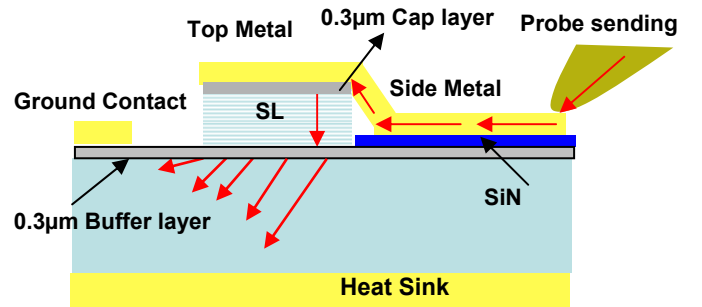
Fig. 2. The structure of a SiGe superlattice micro refrigerator device.
