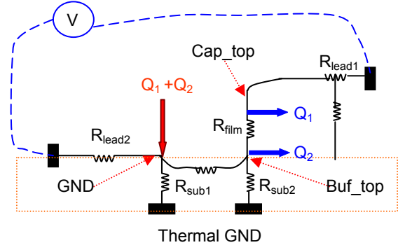
Fig. 4. The thermal circuit of the micro cooler device.
