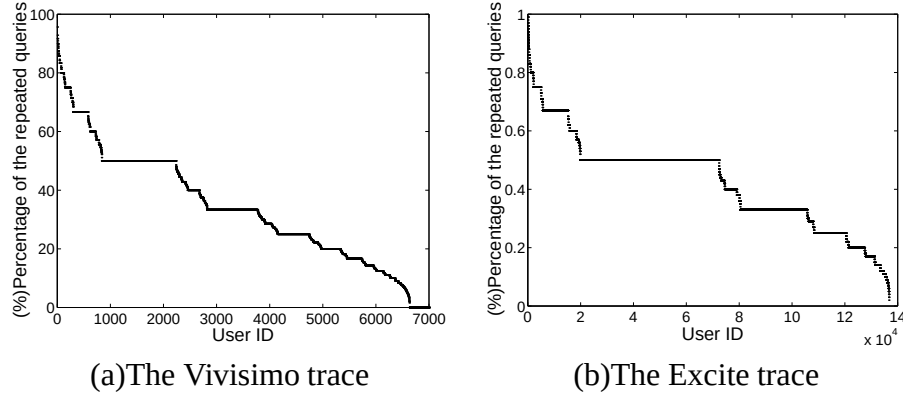
Figure 3: The percentage of the repeated queries over the number of queries submitted by each user (Only those users who repeated queries are plotted here).
