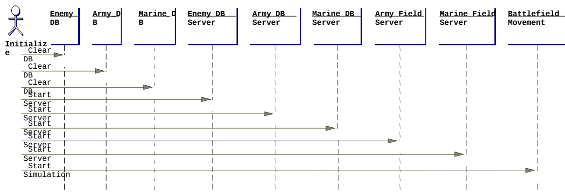
Figure 2-18. Initialization Process
