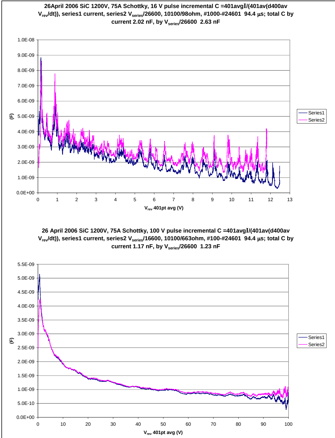
Figure 2. C for SiC Schottky diode at pulsed -16\text{ V} through -600\text{ V} .
