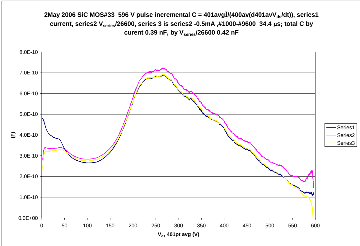
Figure 6. C for SiC MOS #33 at pulsed V_{\text{ds}} of 14.7 V through 596 V (cont'd).
