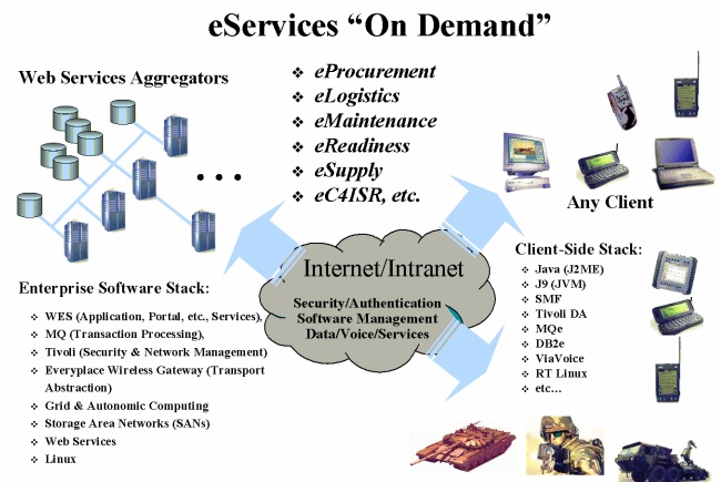
Figure 2: The IBM Middleware Software Stack
