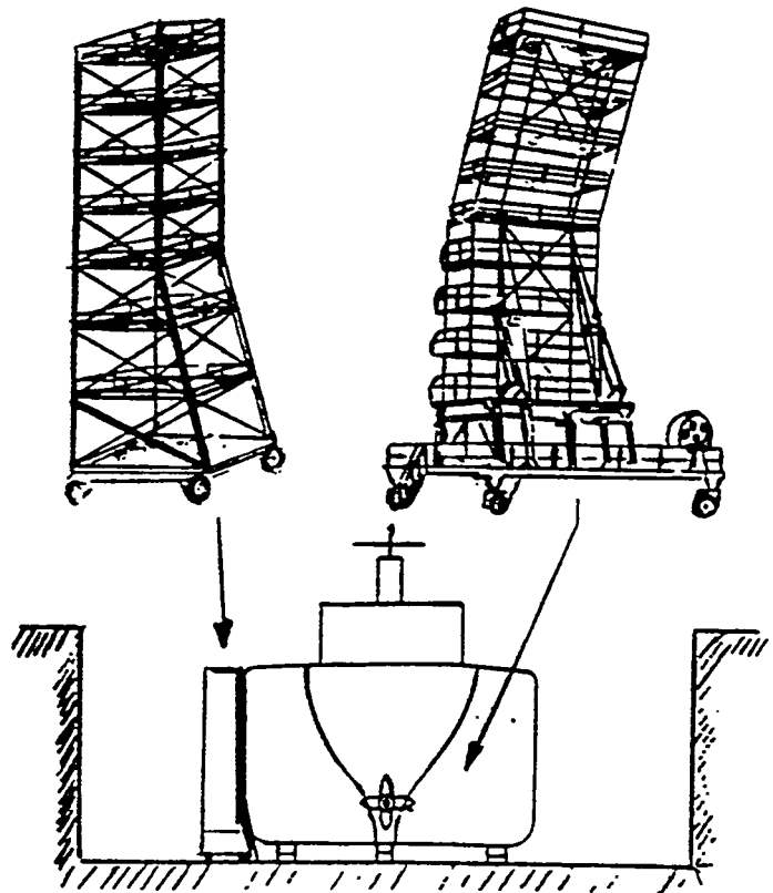
MECHANICAL ROLLING TOWERS USED AT IHI OF JAPAN
