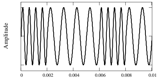
b. Frequency modulated digital signal aka Frequency shift keying
