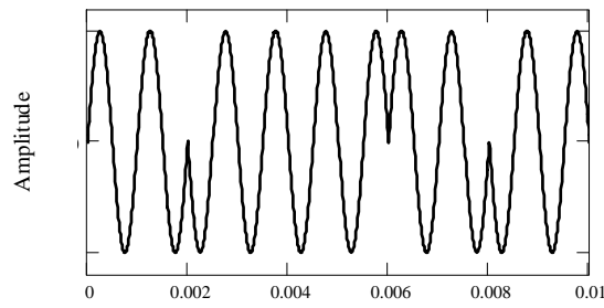
c. Phase modulated digital signal aka Phase shift keying
