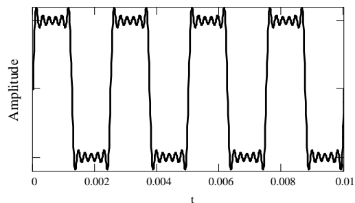
c. Square wave reproduction using frequency components beneath 5 kHz
