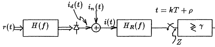
Figure 1: Receiver structure: Optical filter - Detector - Electric low pass filter. \rho(< T) is the time shift required to maximize the received signal energy.
