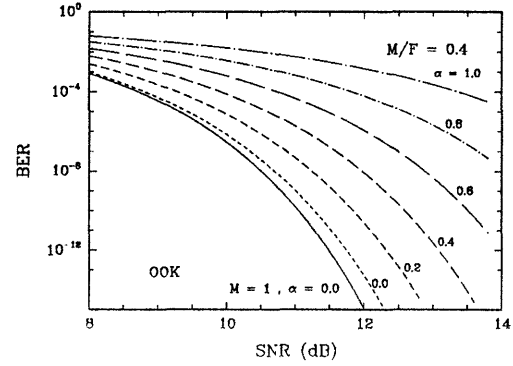
Figure 5: BER crosstalk induced degradation with an FP filter with M/F = 0.4 . Also shown for comparison is the BER curve for one channel (no crosstalk).
