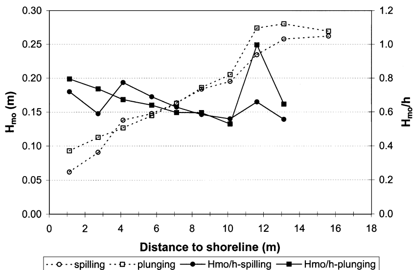
Fig. 2. Cross-shore distribution of significant wave height and breaker index defined as H_{mo}/h .
