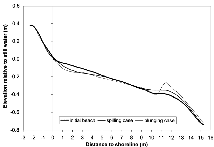
Fig. 4. Initial and equilibrium beach profiles for the two wave cases.
