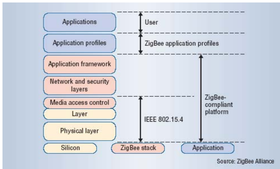
Figure 5. IEEE 802.15.4 and ZigBee working model (Le, 2005).
