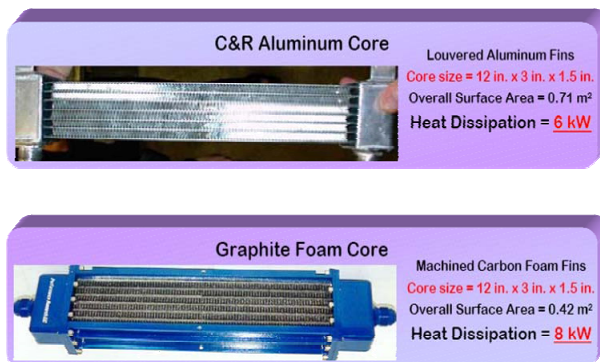
Figure 3: Automotive radiators which demonstrated 33 to 250% performance improvement.
