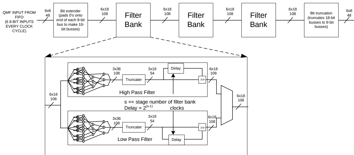
Figure 19. 6 Parallel Input QMF
