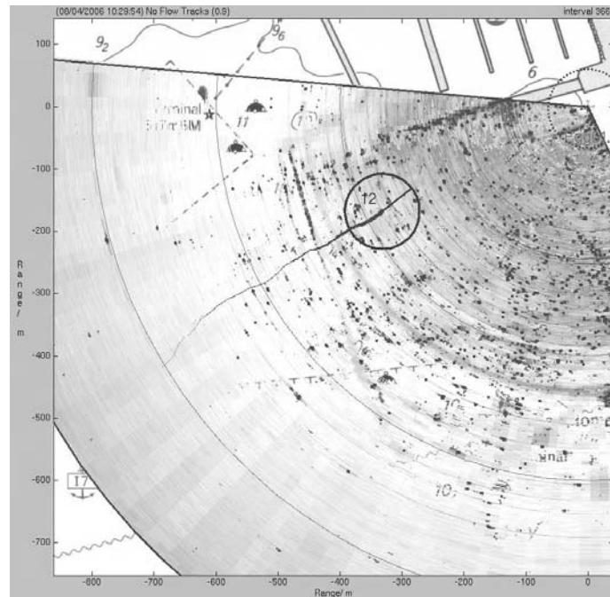
Figure 1. Example (QinetiQ's Cerberus system) of an echograph overlay on chart view near La Spezia. A single intruder is automatically detected and tracked starting in this case at a range of about 800 m from the sonar. A boat wake can be seen near the intruder.
