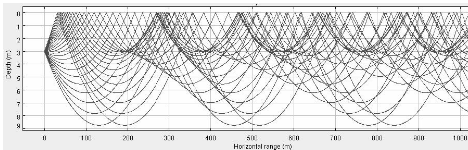
Figure 2. Example of refracted ray paths for sound transmitted by a sonar on the left (at 3 m depth and 0 m range). The water is upward refracting in this case, giving better detection and tracking against intruders near the surface (0 m depth) than near the sea floor 9 m depth. This illustrates one of many possibilities.
