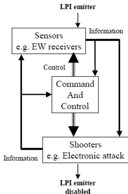
Figure 59. LPI Radar Jamming with Network-Centric Architecture 65
