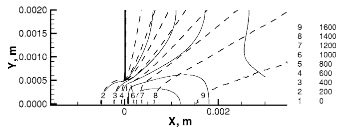
FIG. 3. Helium axial velocity (m/s) at P_0=410 Pa obtained by kinetic (dashed lines) and continuum (solid lines) approaches, t/d=0.015 .
