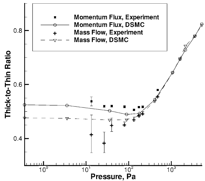
FIG. 11. Ratio of the mass flow and momentum flux for t/d=1.2 to the corresponding values at t/d=0.015 . Helium flow.
