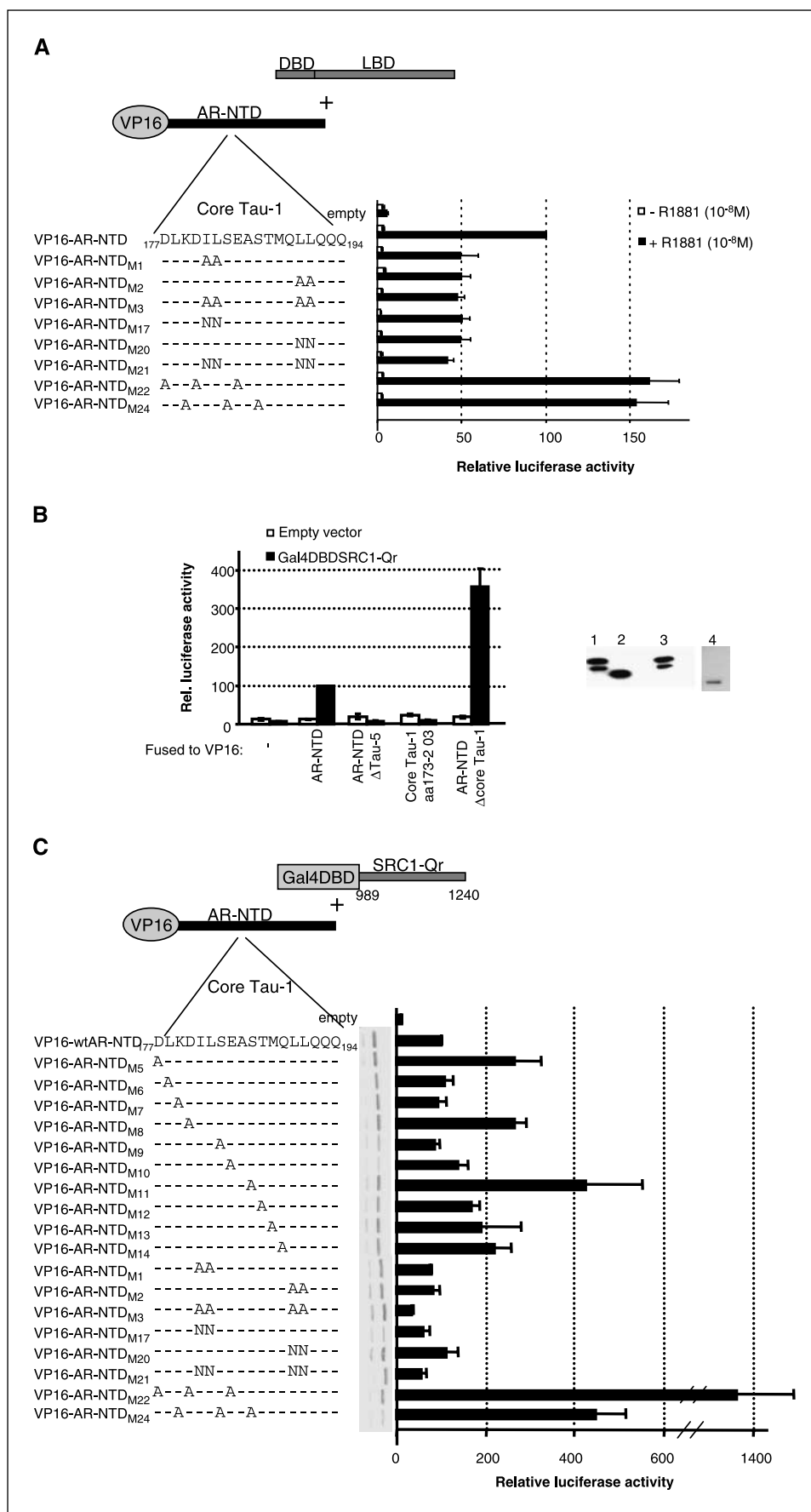
Figure 5. A, two-hybrid assay for the interaction between AR-NTD and AR-LBD. pSG5AR-DBD-LBD (aa 538-919; 50 ng/well) was coexpressed in COS-7 cells with either the empty pSNATCH-II expression vector encoding the activation domain of VP16 or the same expression construct containing the wild-type NTD or mutant NTDs fused to it (50 ng/well). Assays were done using the 2×TAT-GRE(E1b)-Luc reporter (100 ng/well) and the CMV-βGal reporter (5 ng/well) in the presence or absence of 10 -8 mol/L R1881. Activities are depicted relative to the activity of the wtAR-NTD construct, which was set to 100. Columns, mean; bars, SE. B-C, effect of core Tau-1 on the interaction of SRC1-Qr with Tau-5. Deletion mutants in the hAR-NTD and their interaction with SRC1-Qr. pABGal4-DBD SRC1-Qr (989-1240; 50 ng/well) was coexpressed in COS-7 cells with 50 ng of either the empty pSNATCH-II expression vector (open columns) or the same expression vector containing the wild-type AR-NTD or the indicated deletion mutants (50 ng/well; black columns). Assays were done using the (Gal4) 5 -TATA-Luciferase reporter (100 ng/well) and the CMV-βGal reporter (5 ng/well). Columns, mean; bars, SE. Western blot analysis of the cell extracts using anti-Flag antibody were done as described in Materials and Methods [lane 1, AR-NTD; lane 2, AR-NTD ΔTau-5 ; lane 3, AR-NTD Δcore Tau-1 ; lane 4, core Tau-1 (aa 173-203)]. Since core Tau-1 fused to the Gal4DBD is a small fragment, a longer exposure was necessary. C, the same analysis for mutated AR-NTDs as done in (B).
