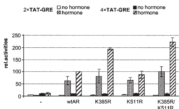
Fig. 7. Effect of Mutation of the SUMO-1 Acceptor Sites on AR Activity on 2×TAT-GRE and 4×TAT-GRE
