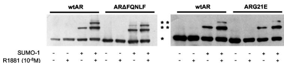
Fig. 4. SUMO-ylation of wtAR, ARΔFQNLF, and ARG21E
