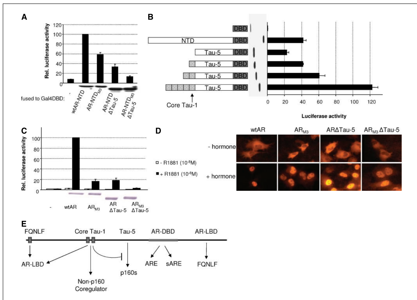
Figure 6. A, abrogating core Tau-1 activity and/or Tau-5 activity leads to a decreased intrinsic activity of the AR-NTD. COS-7 cells were transfected with 50 ng of empty pABGal4, pABGal4AR-NTD or its (deletion) mutants, together with the luciferase reporter construct (Gal4) 5 -TATA-Luc (100 ng/well) and the CMV-βGal reporter (5 ng/well). Activities are depicted relative to the activity of the wtAR-NTD construct, which was set to 100. Columns , mean; bars , SE. Western blot analysis of the cell extracts containing Gal4AR-NTD and fragments using antiGal4DBD antibody was done as described in Materials and Methods. B, core Tau-1 and Tau-5 are both necessary for the full intrinsic activity of the hAR-NTD. Left , COS-7 cells were transfected with either an expression vector for the AR-DBD, the AR-NTD-DBD, Tau-5-DBD or with an increasing number of core Tau-1 copies fused to the Tau-5-DBD (50 ng/well). Assays were done using the 2×TAT-GRE(E1b)-Luc reporter (100 ng/well) and the CMV-βGal reporter (5 ng/well). Columns , mean; bars , SE. Western blot of the cell extracts was done as described in Materials and Methods. C, both core Tau-1 and Tau-5 are necessary for the activity of the full-length AR in the presence of hormone. COS-7 cells were expressed with an expression vector containing the wild-type or the indicated mutated ARs (10 ng/well). Assays were done using the 2×TAT-GRE(E1b)-Luc reporter (100 ng) and the CMV-βGal reporter (5 ng/well) in the presence or absence of 10 -8 mol/L R1881 ( open or black columns , respectively). Columns , mean; bars , SE. Western blot of the cell extracts was done as described in Materials and Methods. D, nuclear localization. COS-7 cells were transfected with the indicated ARs. After 1 hour of stimulation, cells were fixed with 3.7% of formaldehyde, permeabilized with Triton X-100 and incubated with the M2 anti-Flag antibody. Immunocytochemical signals were detected by incubation with a TRITC-labeled secondary antibody. E, model of the complex interplay of several domains in the AR. See text for details.
