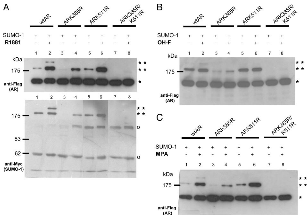
Fig. 1. Analysis of the Ligand Dependency of the Two SUMO-1 Acceptor Sites
