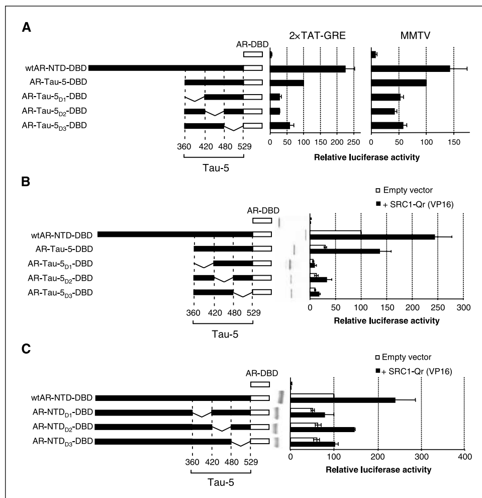
Figure 2. Deletion analysis of the transcription activation function Tau-5. A , Tau-5 as an autonomous transcription activation function. Left , COS-7 cells were transfected with either an expression vector for the AR-DBD, AR-NTD-DBD, or AR-Tau-5-DBD fragments (50 ng/well). As reporter constructs, 2xTAT-GRE(E1b)-Luc (100 ng/well) and the CMV-βGal (5 ng/well) were used. Activities are depicted relative to the activity of the AR-Tau-5-DBD construct, which was set on 100. Columns , mean; bars , SE. For Western blot analysis of the cell extracts, see (B). B-C , two-hybrid assays for the interaction between AR-Tau-5-DBD (B) or AR-NTD-DBD (C) deletion fragments and SRC1-Qr. COS-7 cells were transfected with the expression constructs ( left ), together with either the empty pSNATCH-II expression vector encoding the VP-16 activation domain ( open columns ) or the same expression vector encoding SRC1-Qr-VP-16 fusion (50 ng/well) ( black columns ). Assays were done using the 2xTAT-GRE(E1b)-Luc reporter (100 ng/well) and the CMV-βGal reporter (5 ng/well). Activities are depicted relative to the activity of the AR-NTD-DBD construct in the absence of SRC1-Qr-VP-16, which was set on 100. Columns , mean; bars , SE. Western blot analysis of the cell extracts containing AR-NTD-DBD and fragments using anti-Flag antibody were done as described in Materials and Methods.
