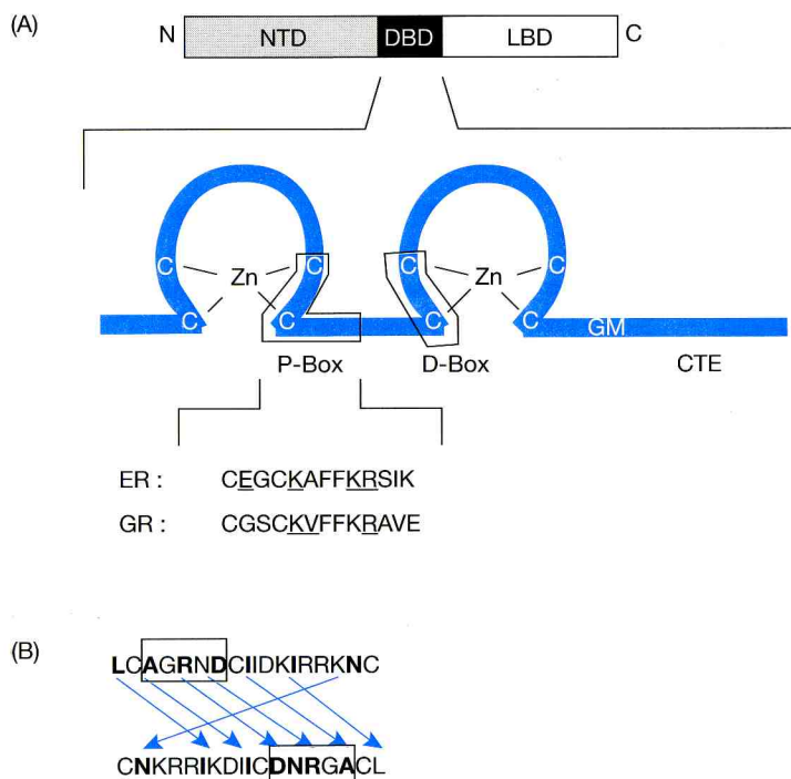
Figure 2. (A) Two types of P-box sequence and (B) GR dimerization interface
