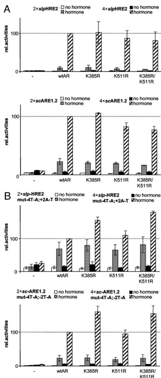
Fig. 8. Synergy Control Motif in AR Transactivation through Canonical vs. Selective HREs
