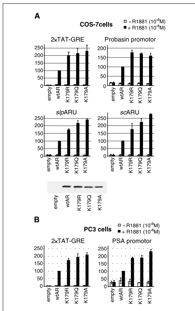
Figure 1. Prostate cancer mutation in the hAR at position 179. A-B, COS-7 (A) or PC3 cells (B) were transfected with an expression vector containing the wild-type or the indicated mutated ARs (10 ng/well). Assays were done using different Luciferase constructs (100 ng/well, top) and the CMV- \beta -Gal reporter (5 ng/well) in the presence or absence of 10^{-8} mol/L R1881 (open and black columns, respectively). Activities are depicted relative to the activity of the wtAR construct in the presence of hormone, which was set on 100. Columns, mean; bars, SE. Western blot analyses of the cell extracts containing wtAR or AR mutations using anti-Flag antibody were done as described in Materials and Methods (A, bottom).
