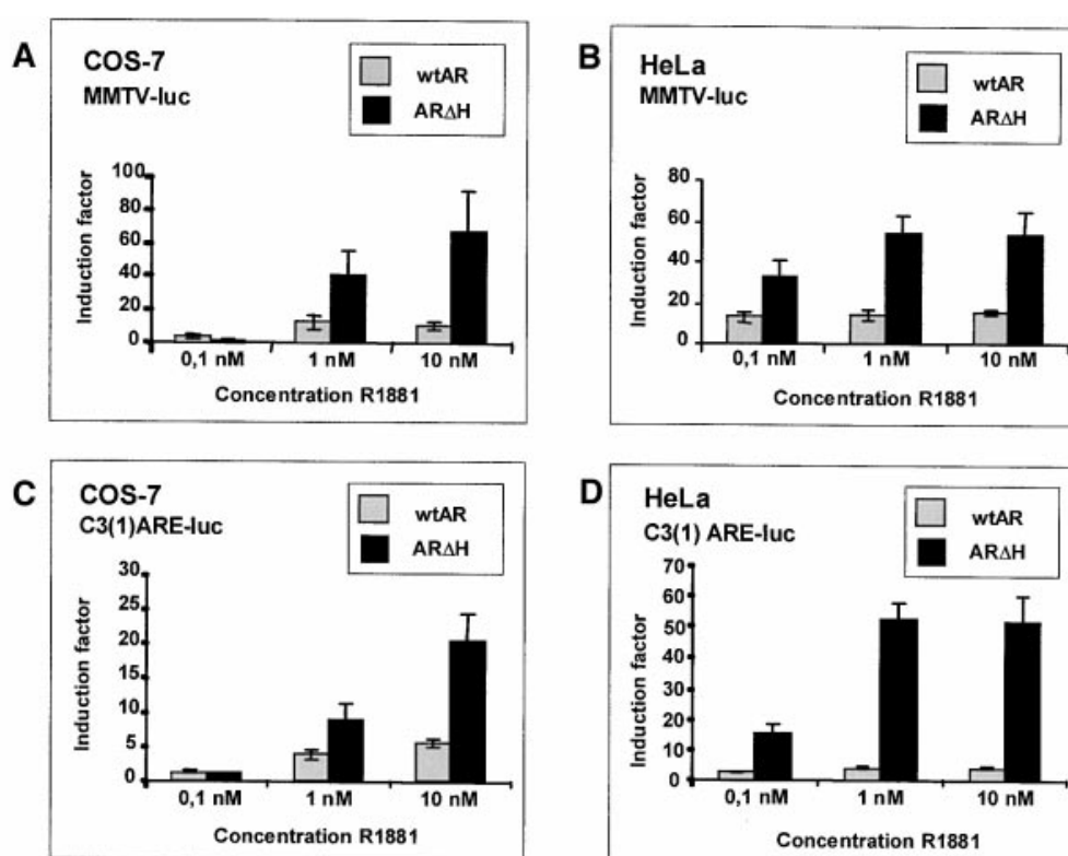
FIGURE 1. The hinge region limits the transactivation potential of the AR at androgen-responsive reporters. COS-7 and HeLa cells were seeded onto 96-well plates at 10^4 cells/well and 1.5 \times 10^4 cells/well, respectively. Twenty-four hours later, cells were transfected with 100 ng of reporter, 10 ng of appropriate receptor, and 10 ng of \beta -galactosidase expression vectors using FuGENE6 reagent (Roche Molecular Biochemicals) according to the manufacturer's instructions. Twenty-four hours after transfection, cells were refreshed with medium with or without androgen (R1881) at the indicated concentrations and incubated for another 24 h, after which cells were lysed with Passive Lysis Buffer (Promega) and assayed for luciferase (Luciferase Assay Reagent; Promega) and \beta -galactosidase (Galacto Reaction Buffer; Tropix, Inc.) activities. The graphs depict induction factors for increasing concentrations of R1881 at two androgen-responsive reporters in both COS-7 cells ( left panels ) and HeLa cells ( right panels ). Reporters used were a luciferase reporter gene driven by the mouse mammary virus long-terminal repeat (MMTV-luc; A and B ) and a luciferase reporter driven by an androgen response element (ARE) of the C3(1) gene of prostate-binding protein [C3(1)ARE-luc; C and D ]. 2 Results represent pooled data from at least three independent experiments with each condition in duplicate.
