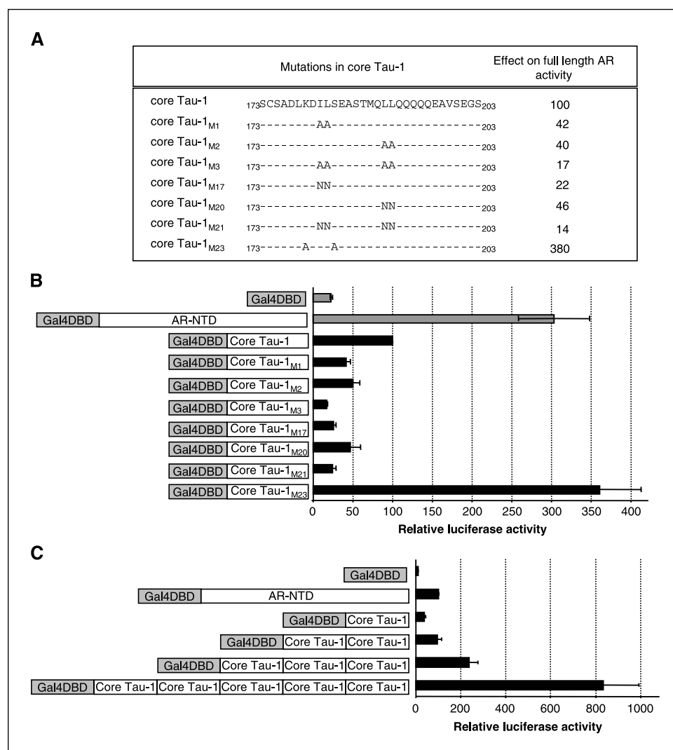
Figure 4. Core Tau-1 of the AR as a strong autonomous transcription activation function. A , schematic representation of the core Tau-1 (aa 173-203) mutants. Left , mutated amino acids in the core Tau-1 region. Right , effect of those mutations on AR activity in the full-length AR, according to the wtAR activity in the presence of hormone (set on 100). B , one-hybrid assay. COS-7 cells were transfected with 50 ng of empty pABGal4 (encoding the Gal4DBD), pABGal4AR-NTD (gray columns), or pABGal4core Tau-1 (wild type or mutated core Tau-1s, black columns), together with the luciferase reporter construct (Gal4) 5 -TATA-Luc (100 ng/well) and the CMV- \beta -Gal reporter (5 ng/well). Activities are depicted relative to the activity of the wild-type core Tau-1-Gal4DBD construct, which was set to 100. Columns, mean; bars, SE. C , one-hybrid assay of multiple copies of core Tau-1. COS-7 cells were transfected and activities were depicted as described in Fig. 4B with the constructs used (left).
