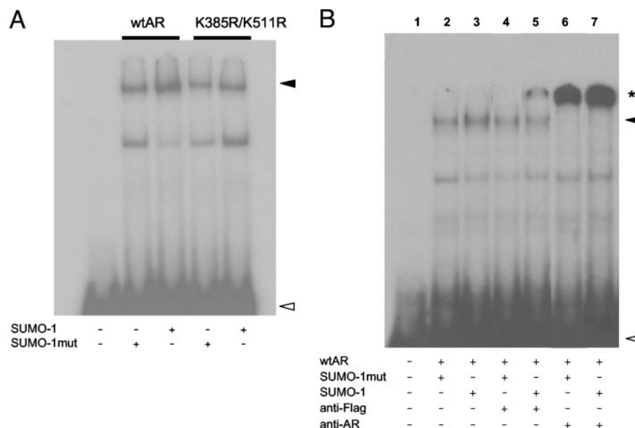
Fig. 5. DNA-Binding Analysis of SUMO-ylated AR
