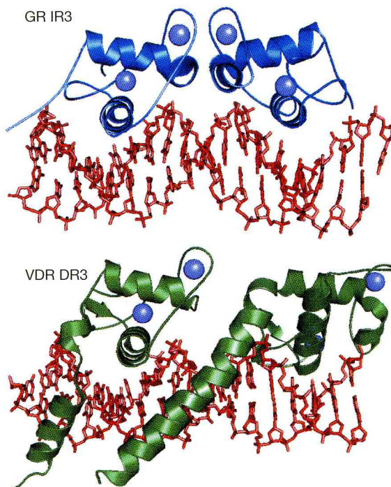
Figure 4. Structure of the GR DBD dimer (blue) binding to a three nucleotide spaced IR (top panel) clearly shows the head-to-head dimerization and the \alpha -helix entering the major groove of the HRE [6]
