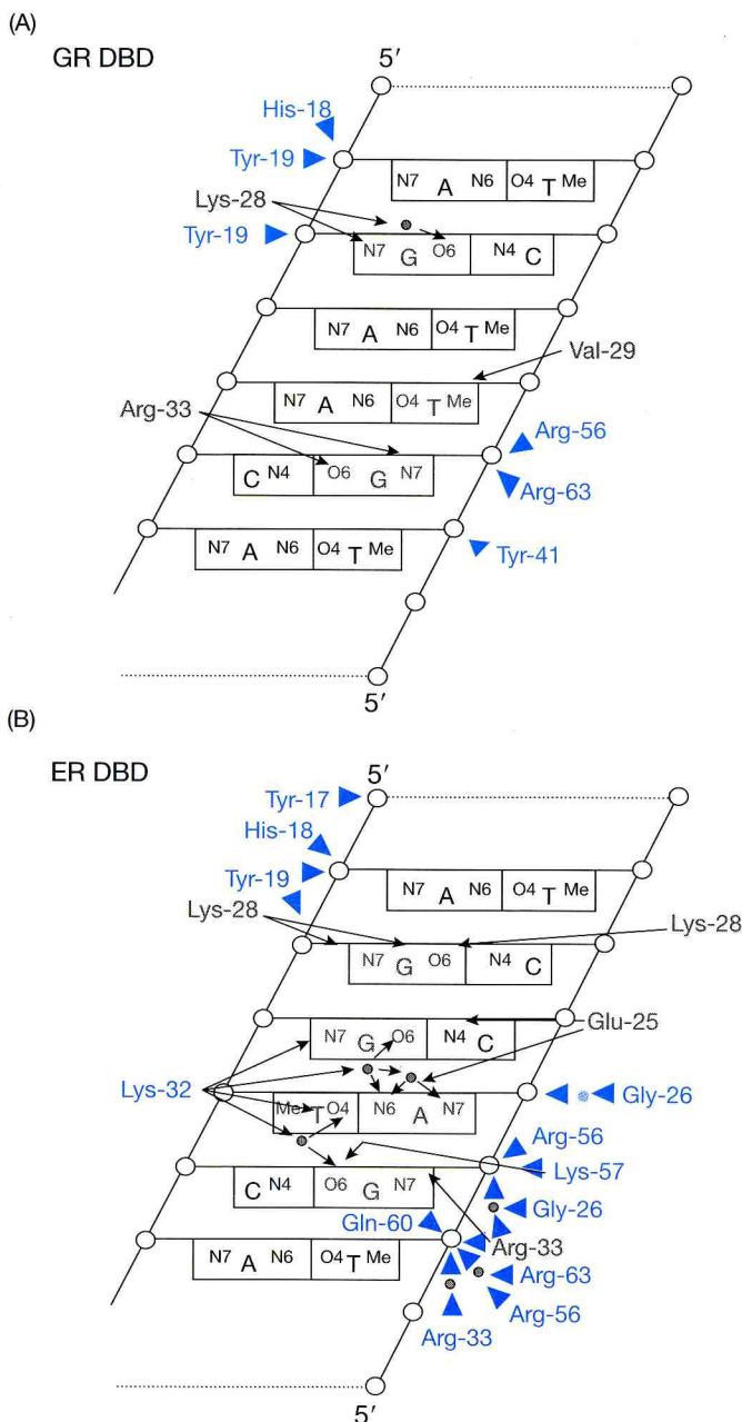
Figure 3. Schematic representation of the protein–DNA contacts between the DNA-recognition helices of the DBDs of GR (A) versus ER (B) to 5'-AGAACA-3' and 5'-AGGTCA-3' respectively
