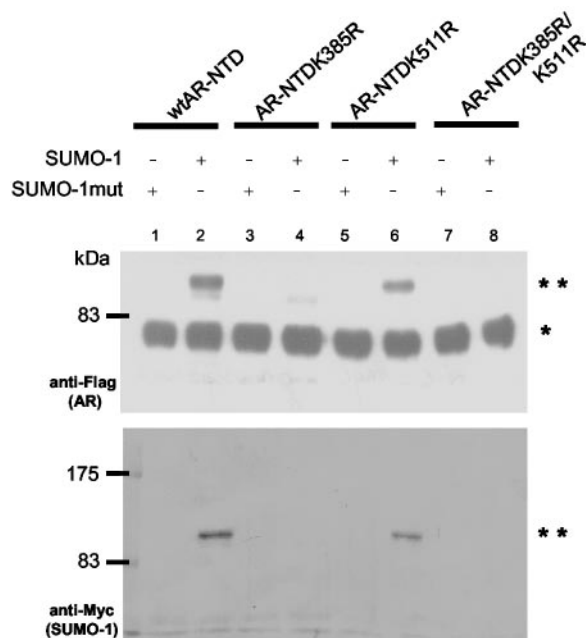
Fig. 3. SUMO-1 Conjugation of ARNTD and Its Mutants COS-7 cells were transfected with Flag-tagged wtAR-NTD, NTDK385R, NTDK511R, or NTDK385R/K511R and co-transfected with c-myc-tagged SUMO-1 or SUMO-1mut. Protein extracts were immunoprecipitated with the anti-Flag antibody agarose, subjected to Western blotting, and probed with the monoclonal M2 anti-Flag antibody ( upper panel ) or anti-c-Myc antibody ( lower panel ). The nonmodified ARs and the SUMO-ylated ARs are indicated on the right by an asterisk or a double asterisk , respectively.
