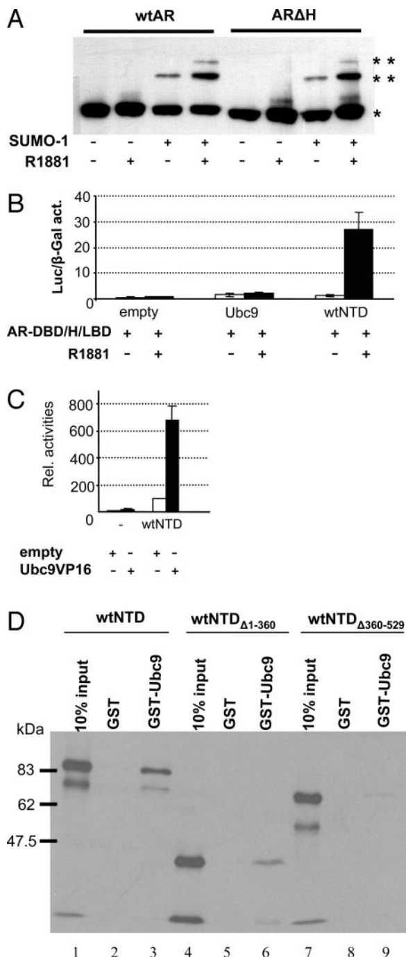
Fig. 2. Ubc9 Interaction with hAR and Effect on AR Activity A , SUMO-ylation of wtAR and ARΔH. COS-7 cells were transfected with Flag-tagged AR or ARΔH and cotransfected with either empty vector pSG5 or with pSG5SUMO-1 and stimulated with or without hormone after 24 h. The extracts were resolved on a 6% SDS polyacrylamide gel and immunoblotted with monoclonal M2 anti-Flag antibody. The positions of nonmodified AR and SUMO-ylated AR are indicated by an asterisk or a double asterisk, respectively. B , Two-hybrid assay. pSG5AR-DBD/H/LBD (538–919aa) (50 ng/well) was coexpressed in COS-7 cells with either the empty pSNATCH-II expression vector or the same expression vector containing Ubc9 or AR-NTD (50 ng/well). Assays were performed using the 2×TAT-GRE(E1b)-Luc reporter (100 ng)
