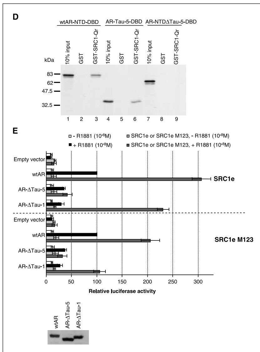
Figure 2 Continued. D, GST pull-down assay. wtAR-NTD-DBD (lanes 1-3) and the AR fragments AR-Tau-5-DBD and AR-NTD \Delta Tau-5-DBD (lanes 4-6 and lanes 7-9, respectively) were transcribed and translated in rabbit reticulocyte lysates in the presence of [ ^{35} S]methionine and incubated with GST or GST-SRC1-Qr beads. Elution was done with SDS sample buffer and analyzed by SDS-PAGE followed by autoradiography. The amount of protein loaded in the input lane is equivalent to 10% of the amount of protein assayed in each binding experiment. E, coactivation of wtAR and deletion mutants with SRC1e or SRC1e M123. Ten nanograms of expression vector for the wtAR, AR- \Delta Tau-5 or AR- \Delta Tau-1 were transfected in COS-7 cells, together with 100 ng of MMTV-Luc and 5 ng CMV- \beta Gal reporter constructs (top). Open and black columns, activity of the AR in the absence and presence of hormone, respectively. Light gray and dark gray columns, values with SRC1e or SRC1e M123 coactivation, in the absence or presence of hormone, respectively. Activities are depicted relative to the activity of the wtAR in the presence of hormone, which was set on 100. Columns, mean; bars, SE. Western blot analysis of the cell extracts containing wtAR and AR deletion mutants using anti-Flag antibody were done as described in Materials and Methods (bottom).
