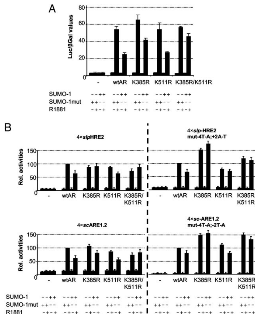
Fig. 6. SUMO-1 Affects AR Activity
