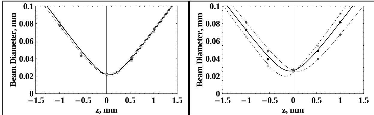
Figure 3. Dependence of beam diameter (by second moment definition) on position along direction of beam propagation after transmitting Bragg grating focused by a lens with f=110 mm. Left – vertical plane; right – horizontal plane. Points – experimental data; curves – fits to Eq. 3. Dashed – transmitted beam; dot-dashed – diffracted beam; solid – combined beam.
