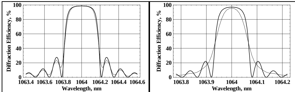
Figure 2. Theoretical spectral dependence of diffraction efficiency for reflecting Bragg gratings with 0.5 nm (left) and 0.2 nm (right) separation from maximum to third zero. Monochromatic plane waves – thick lines; Gaussian beam with divergence of 2 mrad ( FWe^{-2}M ) – thin lines.
