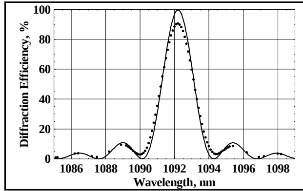
Figure 1. Spectral dependence of diffraction efficiency of a transmitting VBG with 2.2 nm spectral selectivity (Half Width to First Zero). Points – experimental data for near-diffraction-limited beam of ~7 mm diameter; curve – modeling for a plane monochromatic wave.
