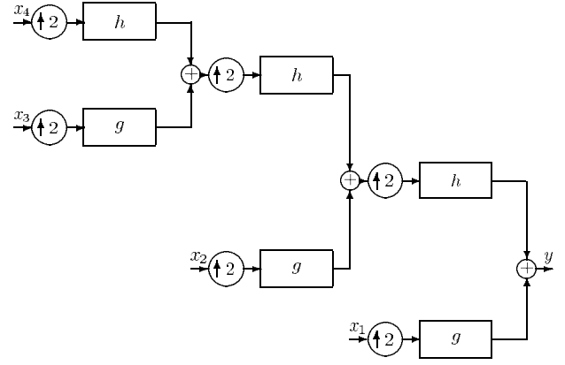
Figure 3: Wavelet Synthesis Filter Bank.
