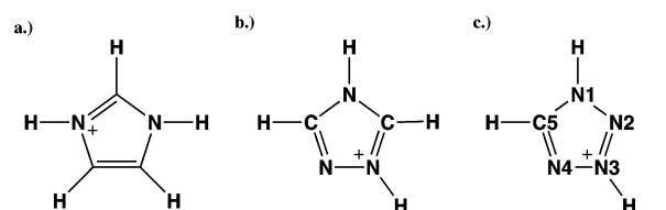
Figure 1. Imidazolium (a), triazolium (b), and tetrazolium (c) cations.
