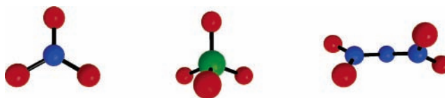
Figure 2. Nitrate, perchlorate and dinitramide anions (oxygen = red, nitrogen = blue, and chlorine = green).
