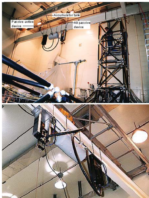
Figure 6 Zero-G suspension system being installed at NASA/Jet Propulsion Laboratory for the Microprecision Interferometer test bed. Top photo shows one passive-active and one all-passive device ganged to support the MPI optics boom. The two devices are connected to a common accumulator tank. Bottom photo is a close-up of the devices. The full system uses three passive-active devices and one all-passive.
