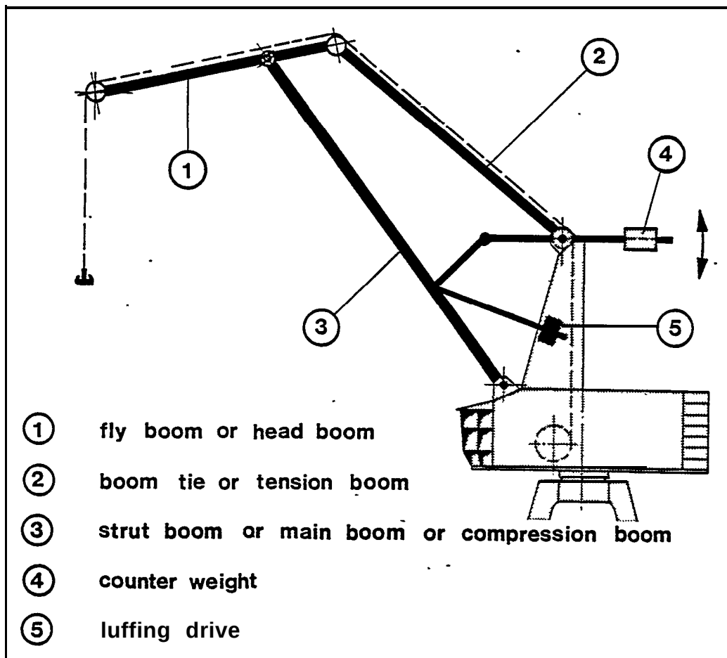
Figure 25: Major Parts of the Double-Boom (Gooseneck) Crane
