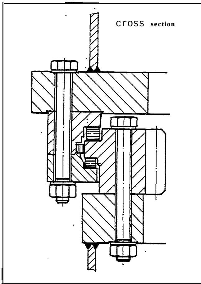
Figure 19: Centerless Roller-Race Bearing
