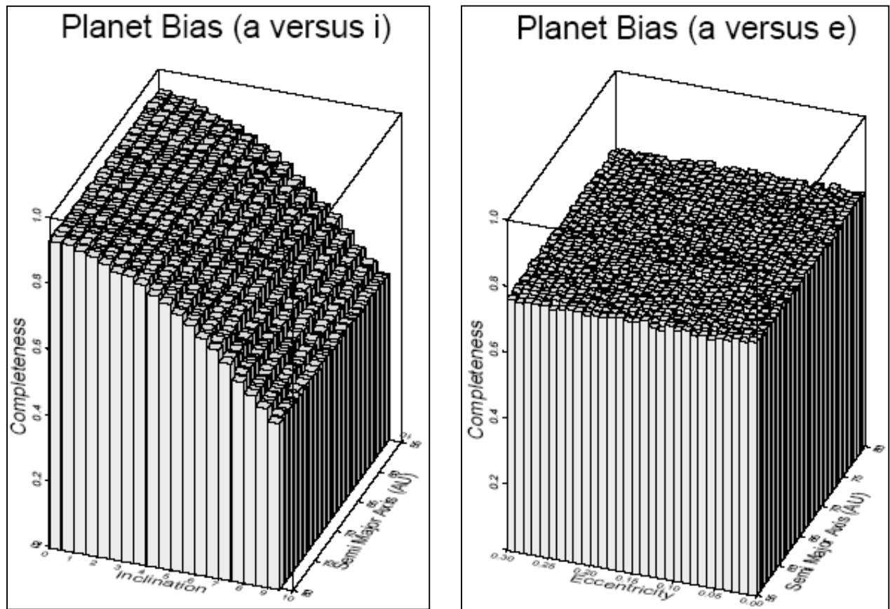
Figure 34: Histograms that represent the percentage of objects detected as a function of semi-major axis versus orbital inclination (left), and semi-major axis versus orbital eccentricity (right) for which the galactic center, monsoon season, and high inclination regions have been excluded. It is still apparent that the orbital inclination, while the eccentricity does not. however, the exclusion of these fields has increased the probability of detection.
