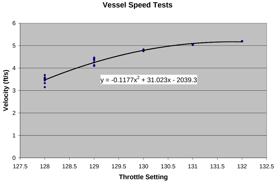
Figure 33: Results of throttle setting tests
