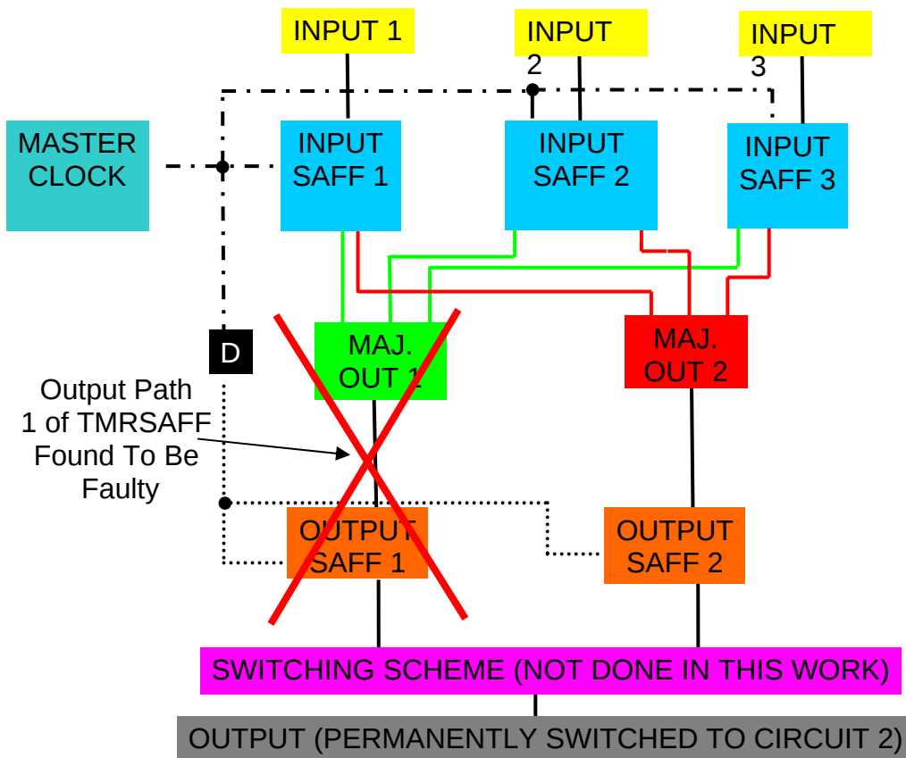
Figure 5.4.4: Self-repairing version of TMRSAFF.
