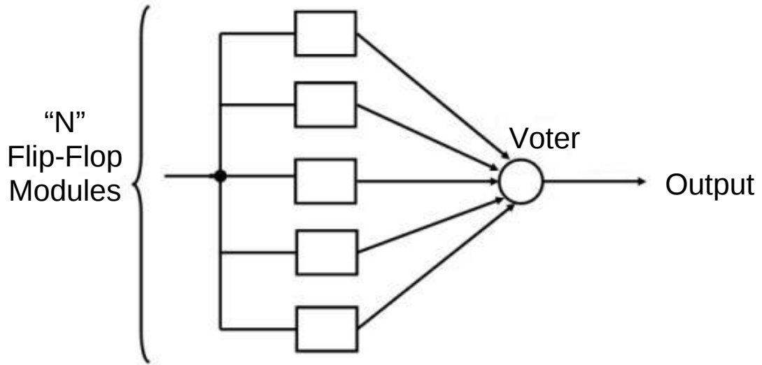
Figure 2.7.1: N-modal flip-flop [12].
