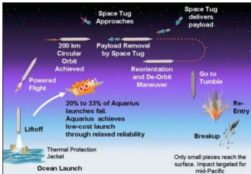
BELOW: Aquarius Mission Profile. Low cost launch is achieved through relaxed reliability. (Source: Space Systems/Loral)
