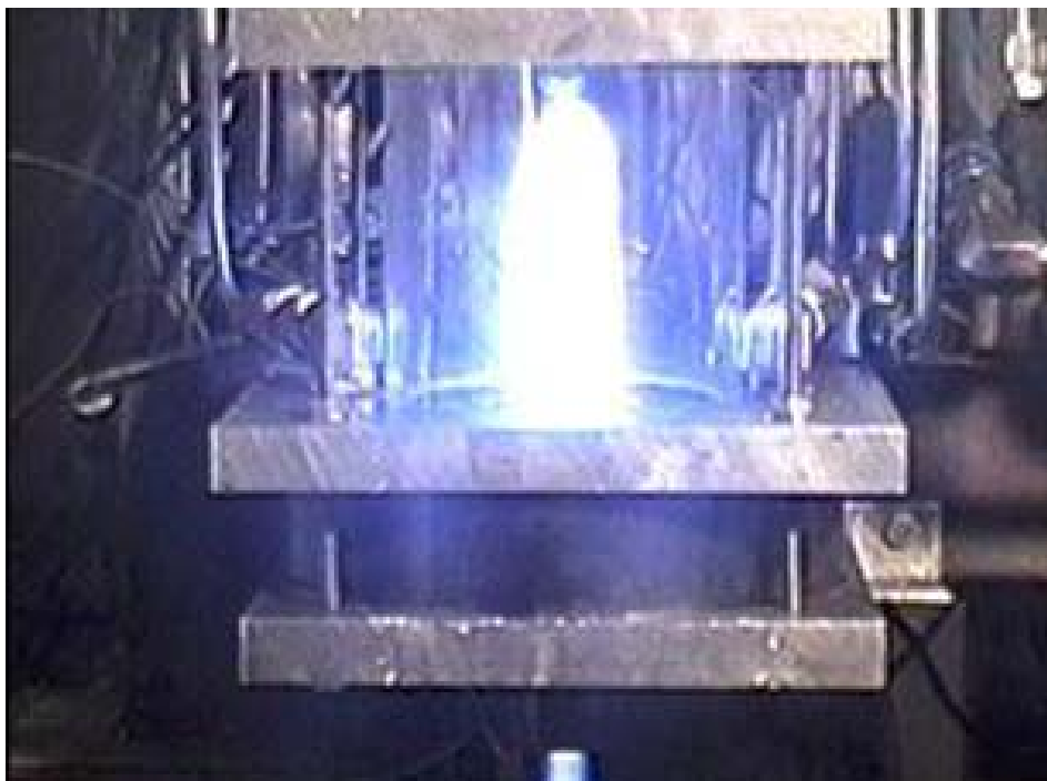
ABOVE: Oxygen and hydrogen burn in a VCCW chamber. The combustion chamber, constructed of Plexiglas, demonstrates the vortex cooled chamber wall concept. The Plexiglas walls remain cool and undamaged even though the temperature in the core vortex is 3000 C. (Source: Orbital Technologies Corporation (ORBITEC™))
