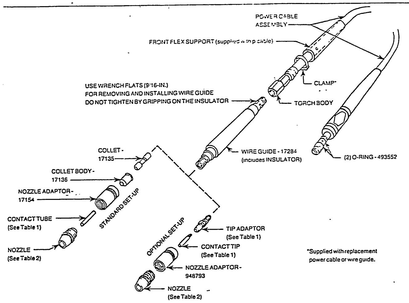
MT-500R Torch Assembly (Liner Not Shown)
