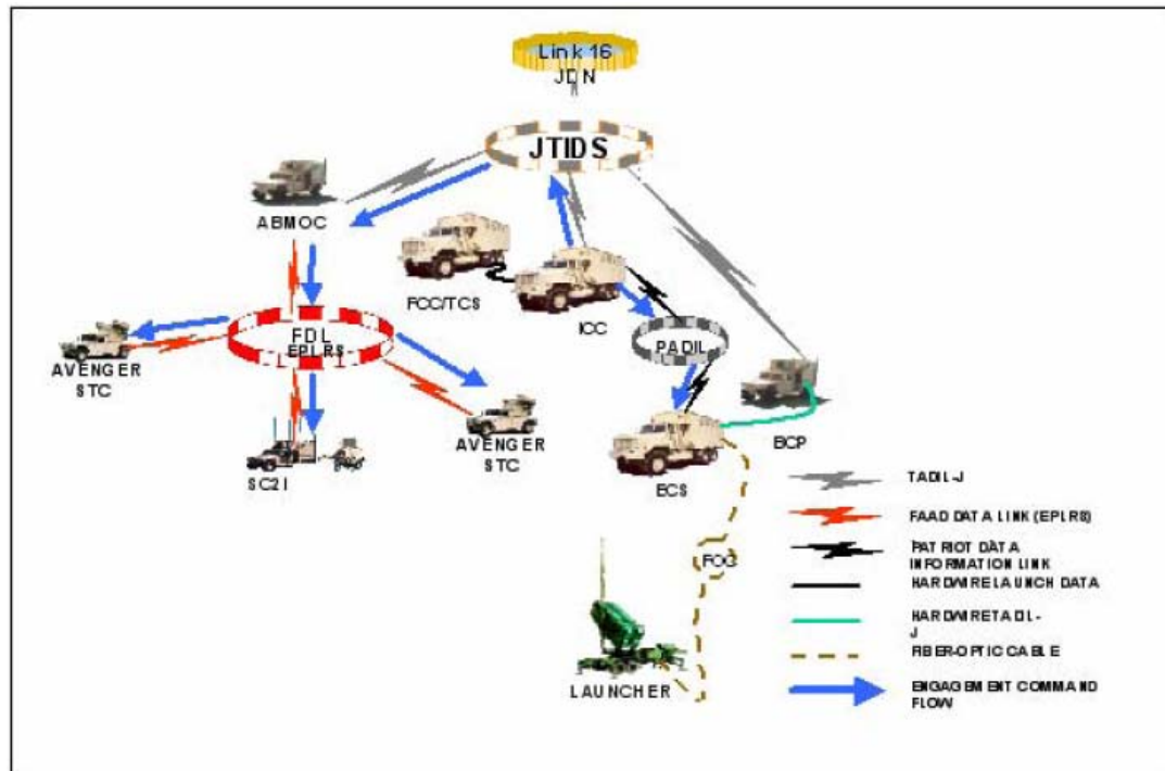
Figure 7. AMD Battalion Data Link Architecture
