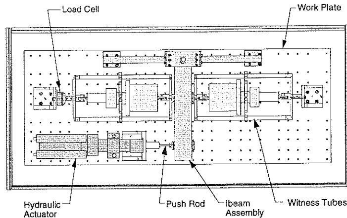
Figure 11. Collinear opposed strut (crosslink) test setup.
